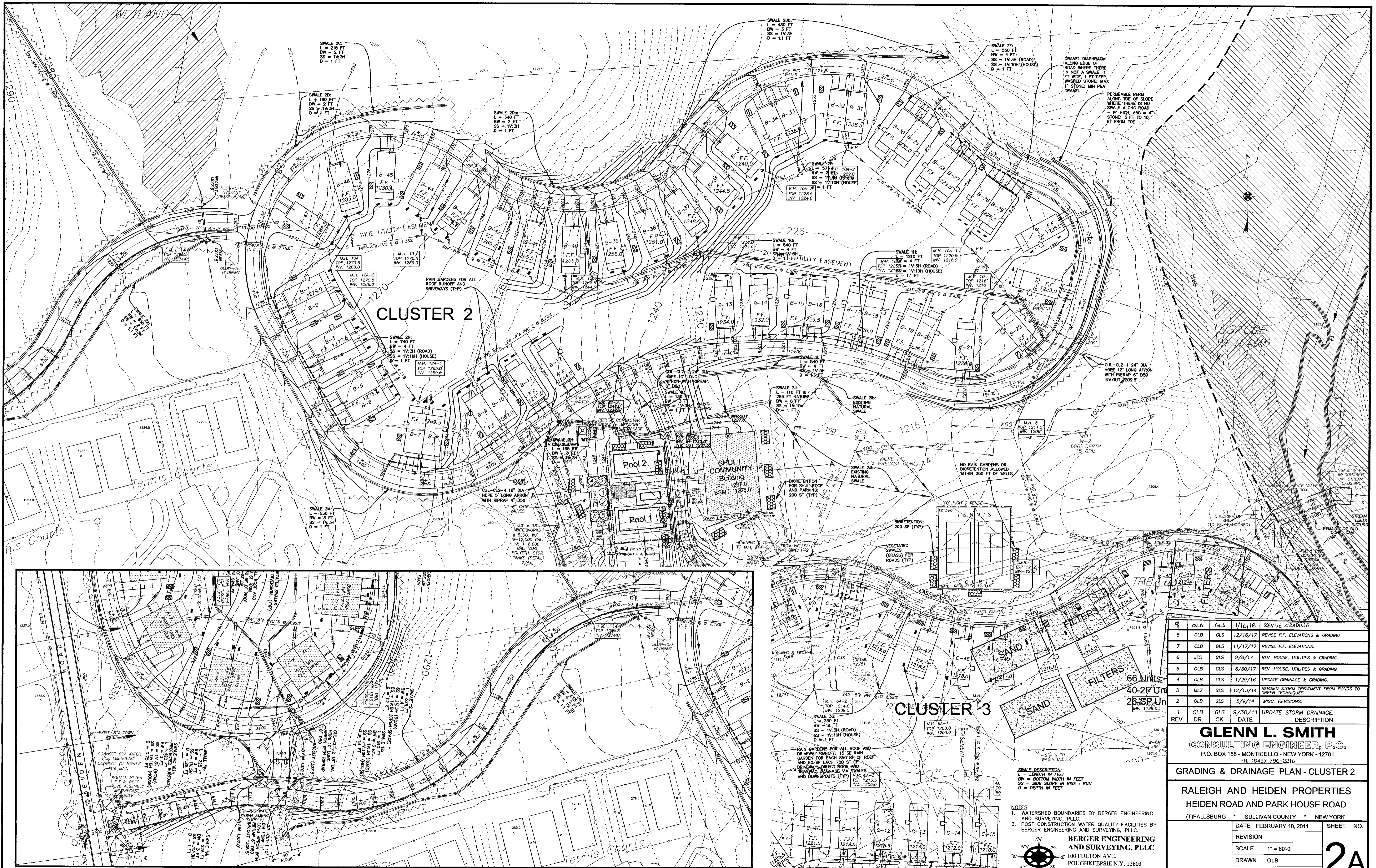
CLUSTER 2 ENTRANCE ROAD FROM HEIDEN ROAD SCALE: 1" = 60'-0"
