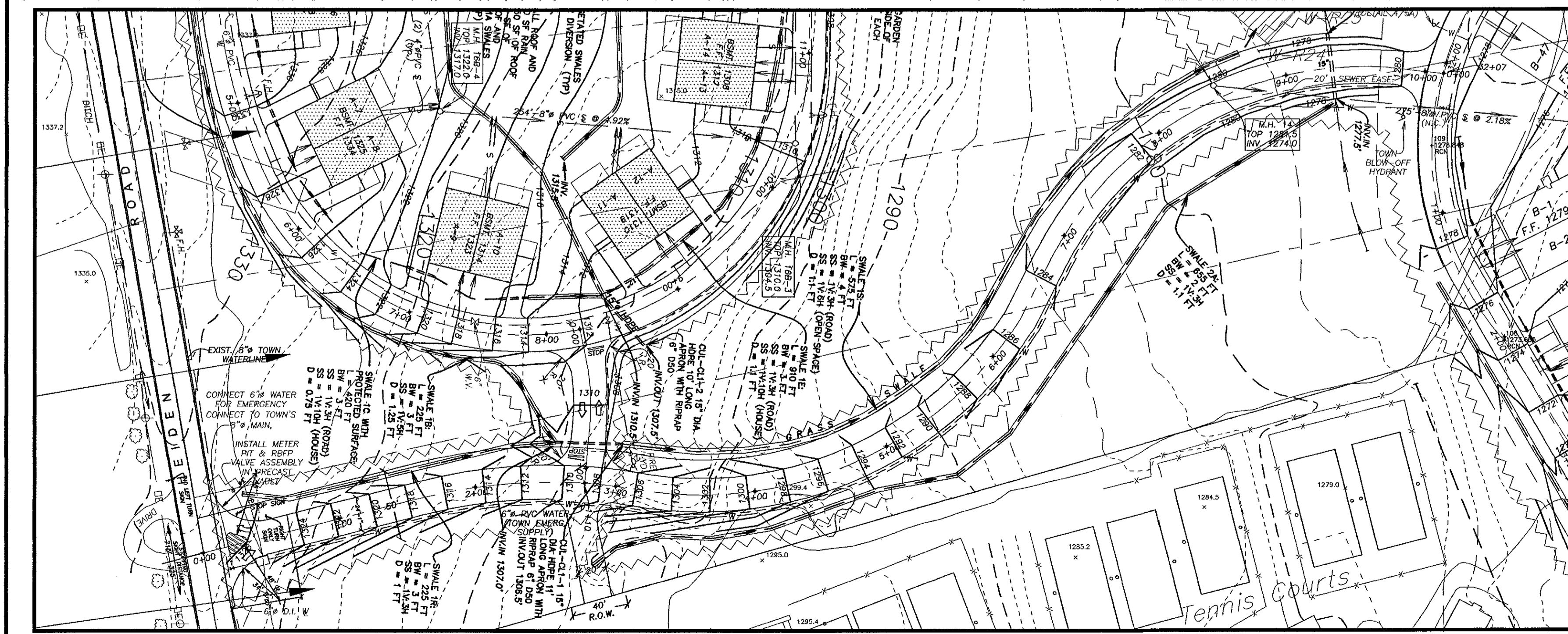
CLUSTER 2 ENTRANCE ROAD FROM HEIDEN ROAD SCALE: 1" = 60'-0"
